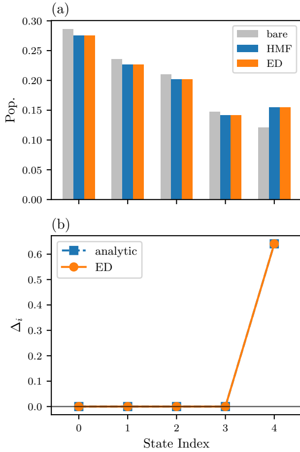
FIG. 4. Microscopic validation. (a) Detailed population snapshot at fixed \beta, g : "Analytic HMF" (blue) corrects the "Bare Gibbs" (grey) to match ED (orange). (b) Effective energy shifts \Delta_i for each level; only the coupled level ( |4\rangle ) shifts, by exactly -\lambda . Non-coupled levels remain unperturbed.
