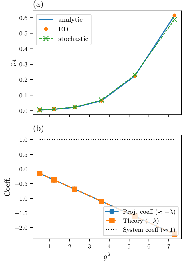
FIG. 3. Strong-coupling benchmark. (a) Population p_4 vs g^2 at fixed \beta , showing excellent agreement over the full range. (b) Coefficients of the HMF in the system basis vs g^2 . The projector component P = |4\rangle\langle 4| scales as -\lambda (orange/blue), while H_S remains unrenormalised (dotted), confirming H_{\text{MF}} = H_S - \lambda f^2 .
